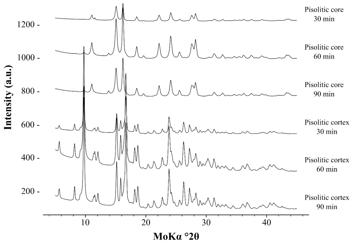
Figure S1: Rotating anode XRD patterns with different exposure times for grain samples from the pisolitic core and cortex of the ferruginous duricrust.
