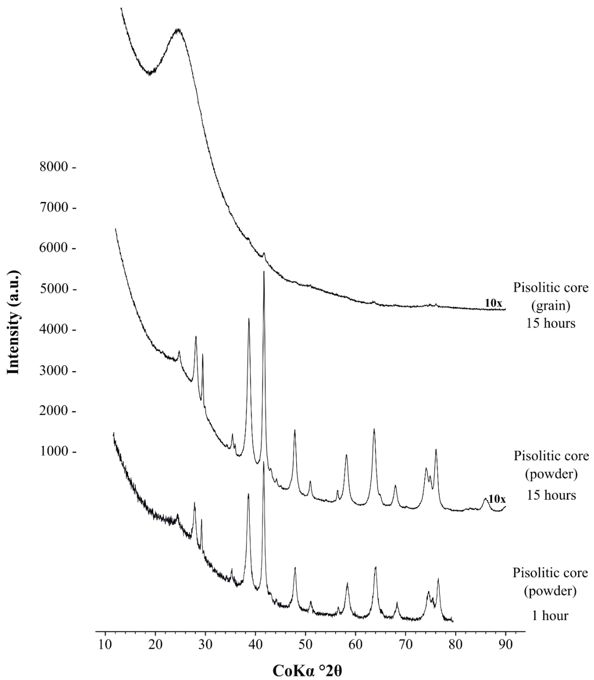
Figure S2: Standard XRD patterns with different exposure times for grain and powder samples loaded in borosilicate capillaries from the pisolitic core of the ferruginous duricrust.
