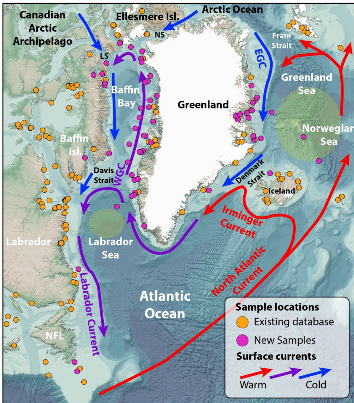
180 Figure 1. Map of Greenland and the northern North Atlantic Ocean, with ocean currents and location of all samples analyzed in this study together with those of the existing \Delta R database (Reimer and Reimer, 2001). Areas of deep convection in the Labrador Sea and north of Iceland are colored yellow. LS: Lancaster Sound, NS: Nares Strait. Bathymetry is from GEBCO (GEBCO Bathymetric Compilation Group, 2022).
