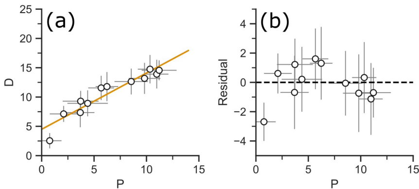
Figure 12. D-P plots for testing for a non-linear relationship. (a) Regression line fit to a synthetic non-linear D-P relationship. (b) Fitting residuals (difference between measured and fitted D).
