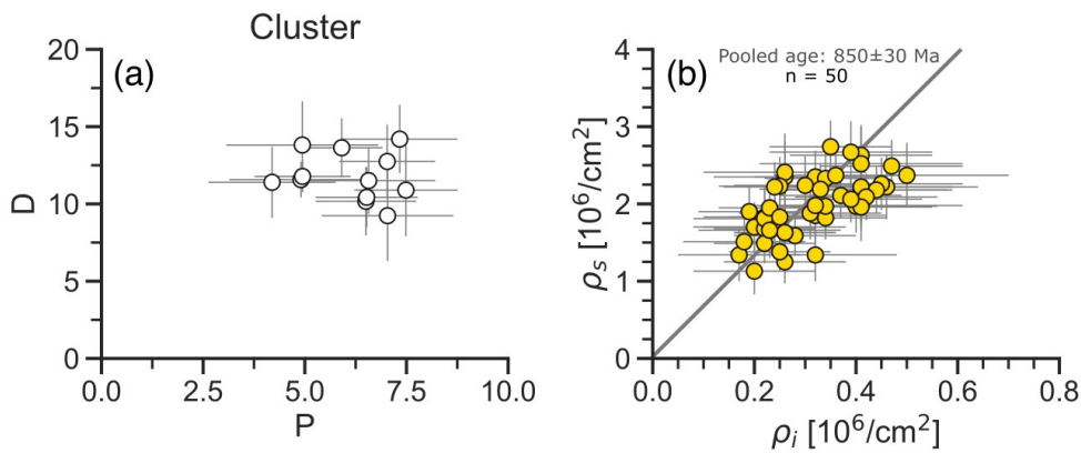
Figure 3. Clustered D-P relationships. (a) D-P plot showing clustered synthetic data. (b) -P plot of apatite fission-track data forming a cluster (FC-1 apatite, Härtel et al., 2022a). The grey line is a tangent through the origin and the mean D and P values representing the pooled age. The uncertainties in b are 2s.
