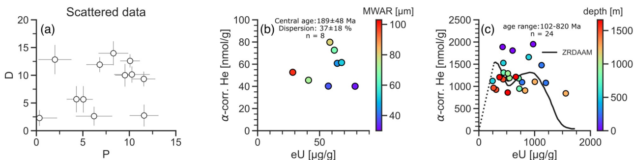
Figure 7. Scattered D-P relationships. (a) D-P plot showing randomly scattered synthetic data. (b) D-P plot of multi-grain-aliquot apatite He data showing a scattered relationship (Shell Canyon 12 sample from Reiners and Farley, 2001). The data are color-coded by grain size expressed as mass-weighted average radius (MWAR). (c) D-P plot of whole-grain zircon He data showing a scattered relationship (Laxemar region samples from Guenther et al., 2017). The line represents the predicted D-P trend from ZRDAAM, and the dotted line segment on the left connects to the origin.
