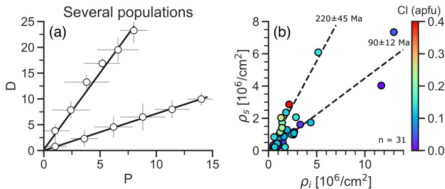
Figure 6. Several-population D-P relationships. (a) D-P plot showing synthetic data with two populations. (b) D-P plot of apatite fission-track data showing two populations (sample I-77, Issler et al., 2005). The data are color-coded by chlorine content (in atoms per formula-unit for \text{Ca}_{10}(\text{PO}_4)_6(\text{F}, \text{OH}, \text{Cl})_2 ). The dashed lines represent ages determined from finite-mixture modelling (Issler et al., 2005).
