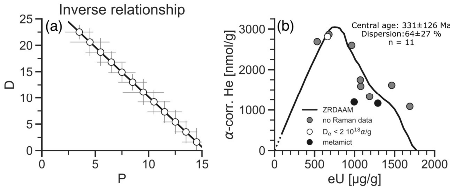
Figure 8. Inverse D-P relationships. (a) D-P plot showing inverse relationship in synthetic data. (b) D-P plot of whole-grain zircon He data showing an inverse relationship (sample A10-42 from Ault et al., 2018, and Armstrong et al., 2024). Color-coding indicates radiation-damage measurements using a Raman microprobe. The line represents the predicted D-P trend from ZRDAAM, and the dotted line segment on the left connects to the origin.
