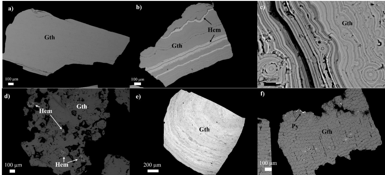
Figure 3. Micrographs of typical grains used in geochronology: a) pure goethite; b) alternate layers of pure goethite and hematite; c) alternate layers of goethite of different chemical composition; d) porous goethite grain containing relic hypogene hematite inclusions; e) pisolithitic goethite; and f) a fragment of fossilized tree trunk showing cells replaced by goethite.
