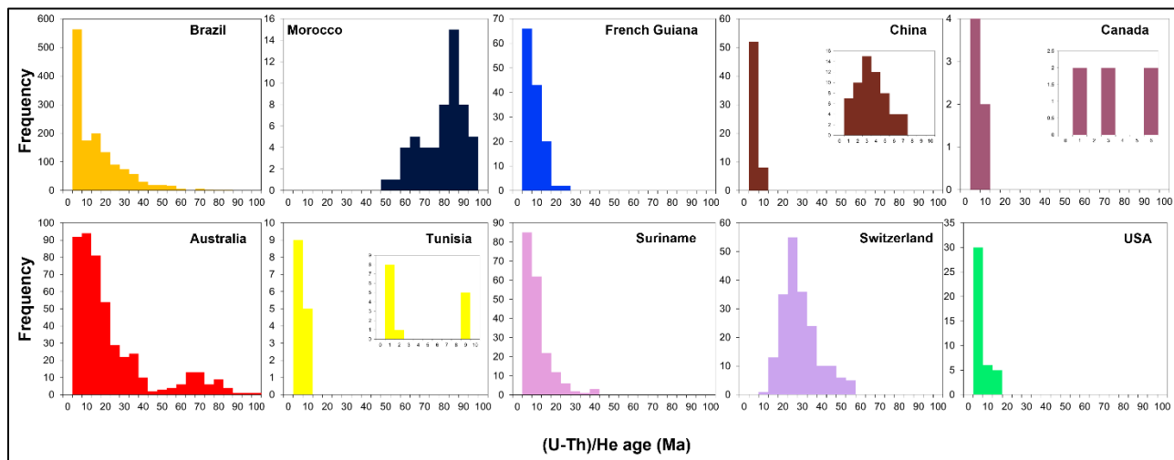
Figure 5. Histograms representing the distribution of goethite (U-Th)/He ages across various regions globally. The histograms offer a detailed insight into the age distribution patterns within each region. Peaks or clusters in the histograms indicate predominant age ranges, while the spread or dispersion of data points provides information on the variability of ages within each region. By combining geographical information with age distribution data, global trends and spatial variations in goethite (U-Th)/He ages show that geological processes and environmental factors influencing the formation and evolution of goethite-bearing weathering profiles differ across the planet.
