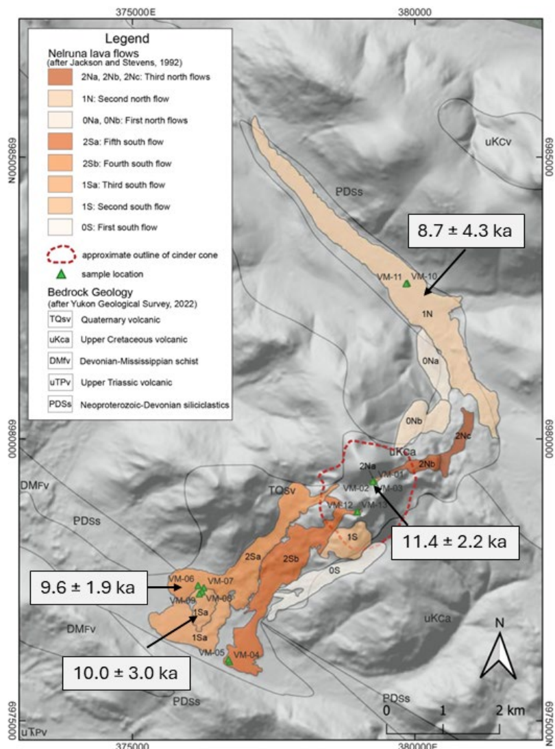
Figure 1. Geologic Map of Volcano Mountain (Nelruna). Map of Volcano Mountain study area after Jackson and Stevens (1992). Samples VM 01,02, and 03 are from the stratigraphically youngest flow on Volcano Mountain, while the other samples all come from flows of very youthful appearance. Numbers in boxes indicate our best estimate of eruption age based on cosmogenic 3 He.
