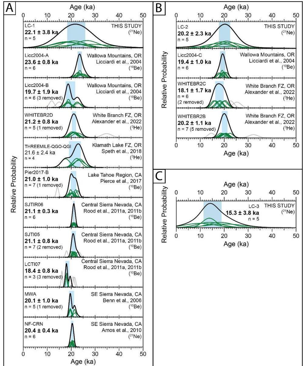
370 Figure 7. Individual and summed pdfs for moraines dated across the Cascade Range and Sierra Nevada. A) Terminal LGM moraine ages from the region listed from north to south (except for the terminal moraine from this study, LC-1, which is listed at the top), B) earliest recessional moraine ages in the region listed north to south, and C) the youngest recessional moraine dated in the LVC (LC-3). For each summed pdf, site (moraine) names from ICE-D, average ages, sample counts (excluding identified outliers noted in parentheses) and citations are reported. Individual ages included in the average age calculation are based on sample ages and internal uncertainties (like Fig. 6) and are plotted in green. Samples that were identified and excluded as outliers using an outlier rejection scheme are plotted in light grey. The solid black line is the summed pdf after outlier removal. The blue box in each plot is the mean and 1 standard deviation of all samples for each moraine. Note that site locations here correspond to site locations and citations denoted in Figure 1.
