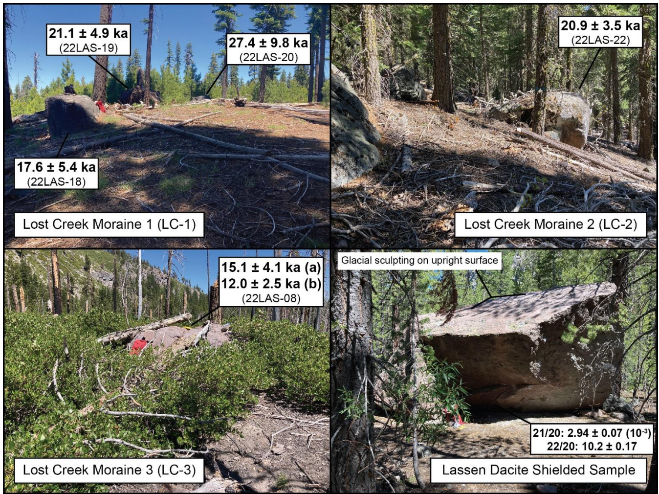
220 Figure 4. Example field sample photos, one per moraine. Clockwise from top left: Three samples clustered nearby on the outermost LGM moraine, Lost Creek 1, one boulder embedded in the Lost Creek 2 moraine, the large block sourced from the dacite of Lassen Peak that was entrained in the 1915 avalanche and debris flow with approximate location of underside sample collection noted, and one boulder with two aliquots measured from the collected surface sample on the Lost Creek 3 moraine. Moraine boulders are shown with calculated ages and internal uncertainties (Photo credits: JP Tulenko).
