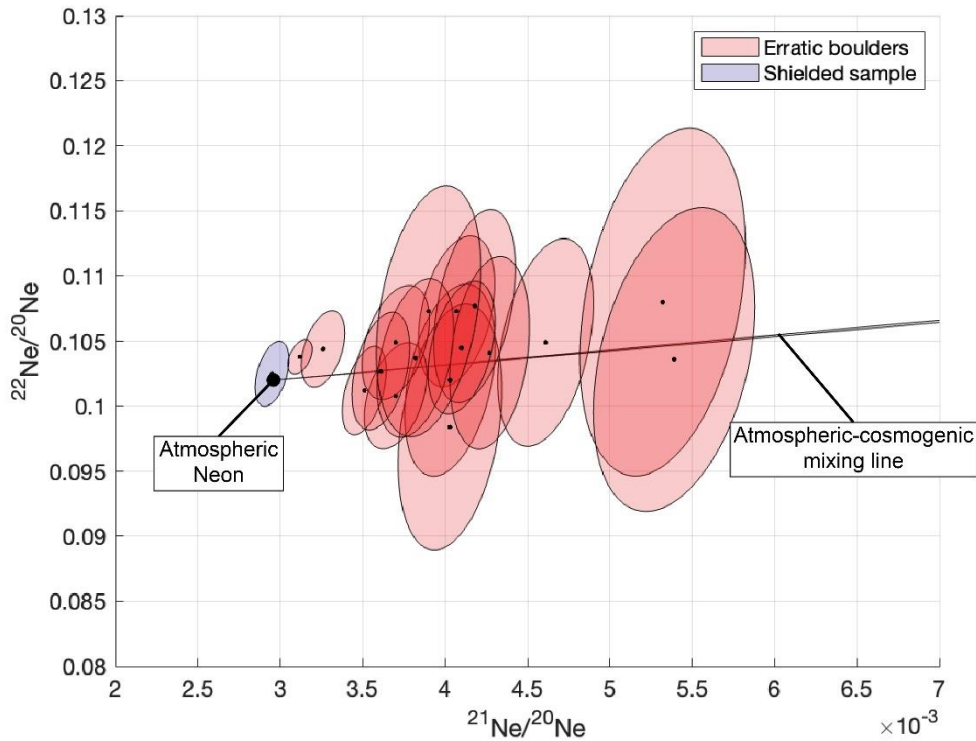
280 Figure 5. Neon three-isotope plot for all 950° C heating steps. The black dot is the composition of atmospheric neon, and the black line is the atmospheric-cosmogenic mixing line (Niedermann, 2002). The ellipses are 68% confidence regions. The isotope composition of neon in the shielded sample is indistinguishable from atmosphere, indicating a negligible concentration of nucleogenic or magmatic neon. All other data lie on or near the atmospheric-cosmogenic mixing line within uncertainty.
