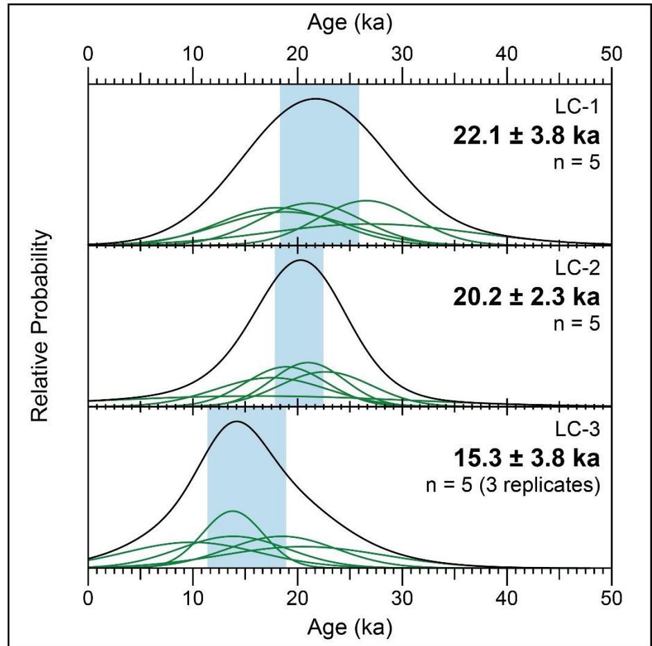
305 Figure 6. Individual probability density functions (pdfs) for each sample (green) and summed pdfs for each moraine age (black). Individual pdfs are based on the calculated age and internal uncertainty for each sample. Blue bars indicate the mean and 1 standard deviation of the ages on each moraine.
