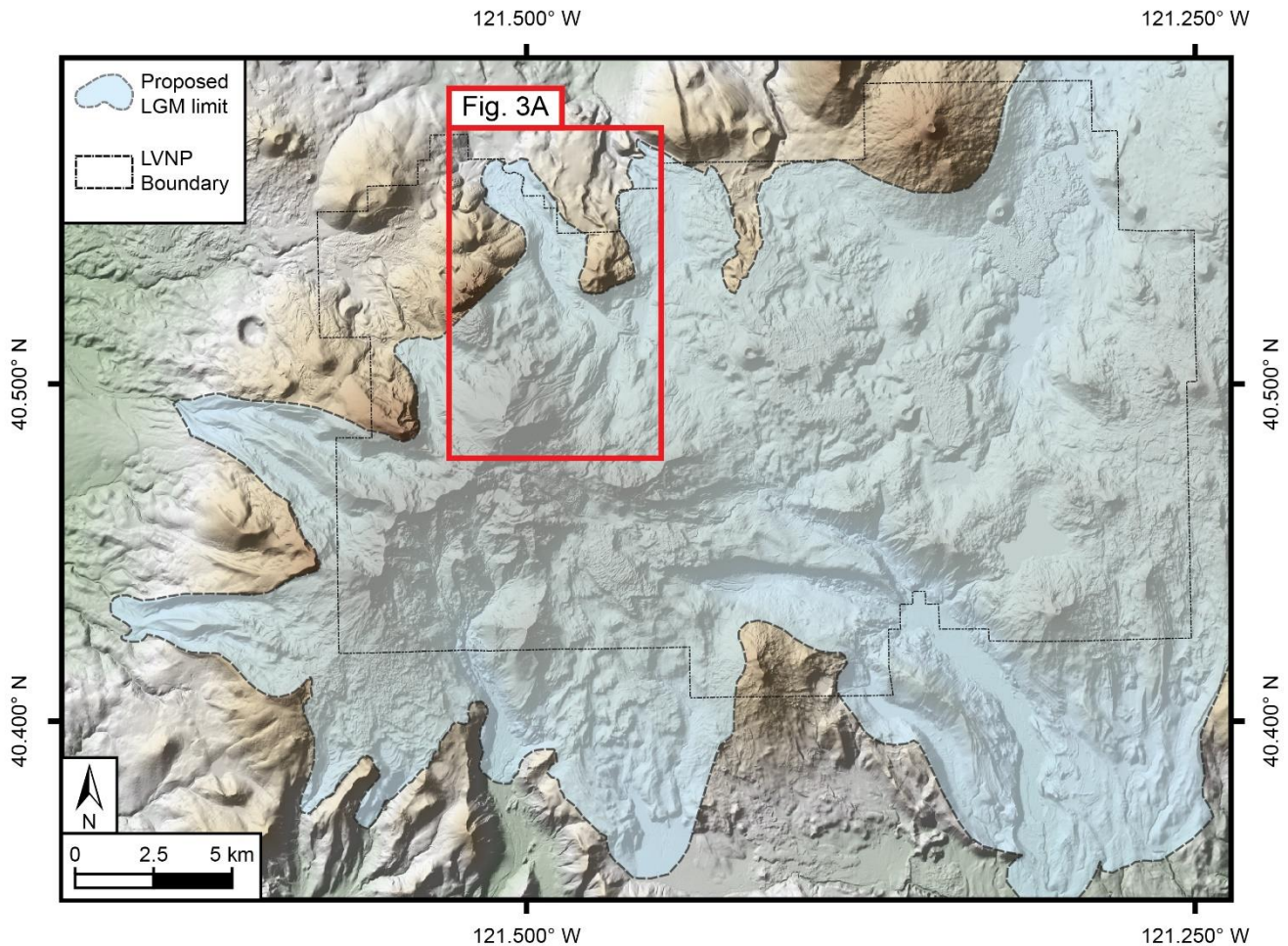
170 Figure 2. Map of Lassen Volcanic National Park and vicinity. Dot-dot-dash lines are park boundary, light blue transparent shade is the proposed limit of LGM glaciation in the region (adapted from Clynne and Muffler, 2010). Basemap and hillshade are from the 1/3 arc-second digital elevation model made available through the USGS National Map 3D Elevation Program ( https://www.usgs.gov/programs/national-geospatial-program/national-map date of last access; Feb 1, 2024).
