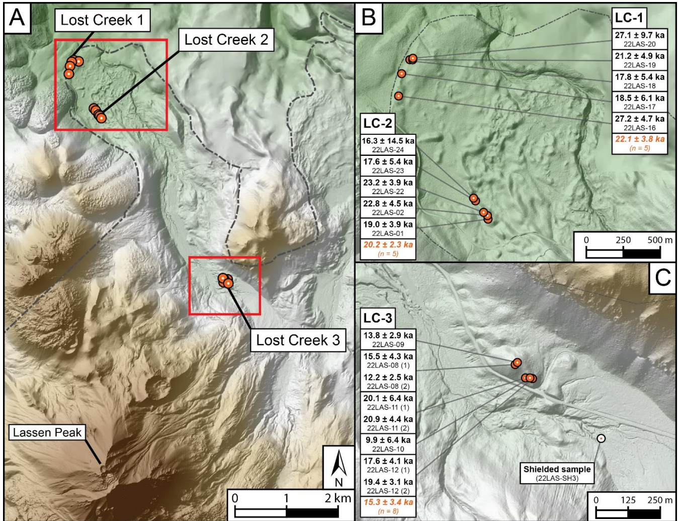
185 Figure 3. Lost Creek drainage north of Lassen Peak. A): A: Lost Creek drainage with sample locations highlighted for each moraine (Lost Creek 1, 2 and 3). B: Zoom in on Lost Creek 1 and Lost Creek 2 (A1) moraines. Samples listed with calculated ages and internal uncertainties. Average moraine ages in orange text. C: Zoom in on Lost Creek moraine 3 (A2) up-valley from Lost Creek moraines 1 and 2. Individual ages and moraine ages reported in the same way as panel B. Note the multiple aliquots measured for samples 22LAS-08, 22LAS-11 and 22LAS-12. Location of the large block entrained in the 1915 avalanche and debris flow used to procure a shielded sample noted in panel C. Basemap and hillshade are sourced from post-processed, Lidar-based digital elevation model products available through the USGS National Map 3D Elevation Program ( https://www.usgs.gov/programs/national-geospatial-program/national-map date of last access; Feb 1, 2024). 190
