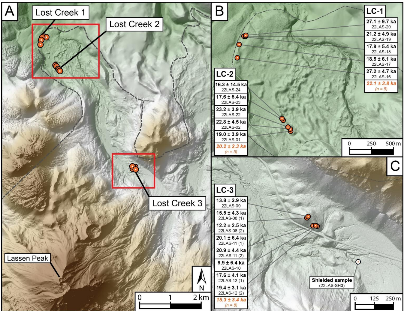
180 Figure 3. Lost Creek drainage north of Lassen Peak. A). A: Complete Lost Creek drainage with sample locations highlighted for each moraine (Lost Creek 1, 2 and 3). B: Zoom in on Lost Creek 1 and Lost Creek 2 (A1) moraines. Samples listed with calculated ages and internal uncertainties. Average moraine ages in orange text. C: Zoom in on Lost Creek moraine 3 (A2) up-valley from Lost Creek moraines 1 and 2. Individual ages and moraine ages reported in the same way as panel B. Note the multiple aliquots measured for samples 22LAS-08, 22LAS-11 and 22LAS-12. Location of the large block entrained in the 1915 avalanche and debris flow used to procure a shielded sample noted in panel C. Basemap and hillshade are sourced from post-processed, Lidar-based digital elevation model products available through the USGS National Map 3D Elevation Program 185 ( https://www.usgs.gov/programs/national-geospatial-program/national-map date of last access; Feb 1, 2024).
