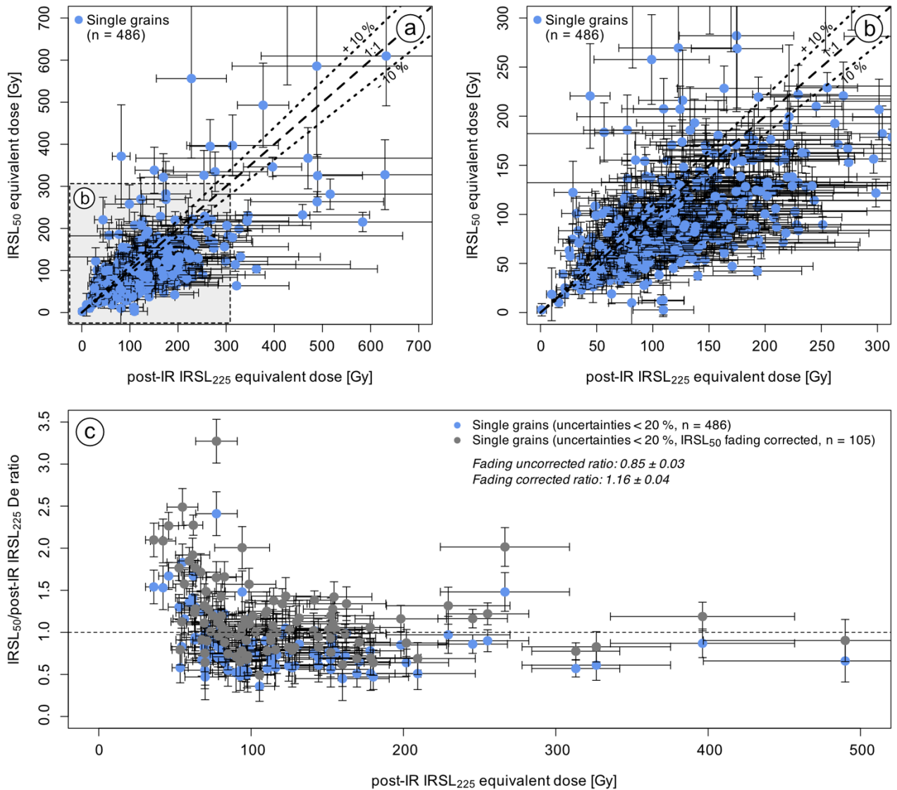
Fig. 34. (a) Scatter plot of post-IR IRSL 225 doses compared to IRSL 50 doses obtained for single grains of all samples . Here the results of single grains of all samples are shown, which passed the acceptance criteria in case of both signals, and which yielded finite equivalent doses. The shaded rectangle shows the region of the plot highlighted in (b). (c) Ratios of IRSL 50 doses divided by post-IR IRSL 225 doses dependent on the size of the post-IRIRSL 225 dose calculated for all data points displayed in (a) which have individual equivalent dose uncertainties <20 % . We chose to limit the display to those grains with the most accurate equivalent doses. The grey points show ratios obtained by dividing the fading corrected IRSL 50 De values by the post-IR IRSL 225 De values (following Thomsen et al., 2008).
