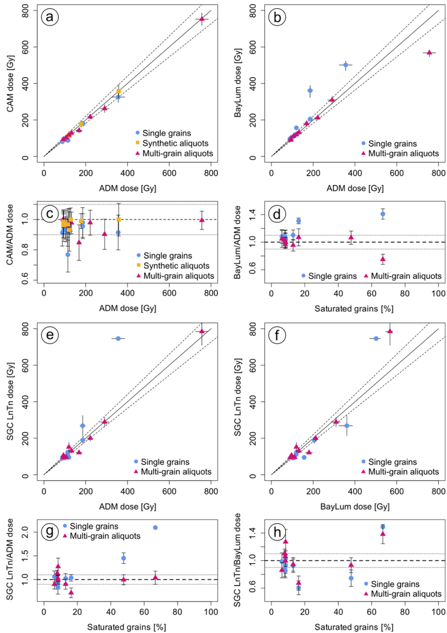
Fig. 45. Comparison of equivalent doses derived using the four dose models for the different dose models and their results for single grains, multi-grain aliquots, and synthetic aliquots. Subfigures (a), (b) and (e) show a comparison of ADM doses and doses obtained using the CAM, BayLum and the SGC L_nT_n method. Subfigure (f) compares BayLum doses to doses calculated using the SGC L_nT_n method. For each dose model comparison the doses resulting from the calculations are visualised as scatter plot of the doses and as ratios dependent on the ADM dose (c) or the percentage of grains in saturation (d,g,h).
