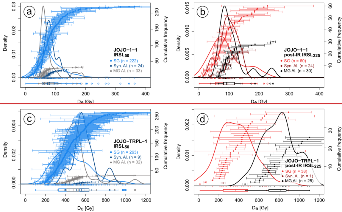
Fig. 3. Kernel density plots (KDE) plots of equivalent dose distributions for the IRSL 50 (a, c) and post-IR IRSL 225 (b, d) signal for the youngest sample JOJO-1-1 (a, b) and the oldest sample JOJO-TRPL-1 (c, d). Only the number of accepted grains/aliquots is displayed in the figure and legend. Dose distributions for single grains (SG), synthetic aliquots (Syn. Al.) and multi-grain aliquots (MG Al.) are shown.
