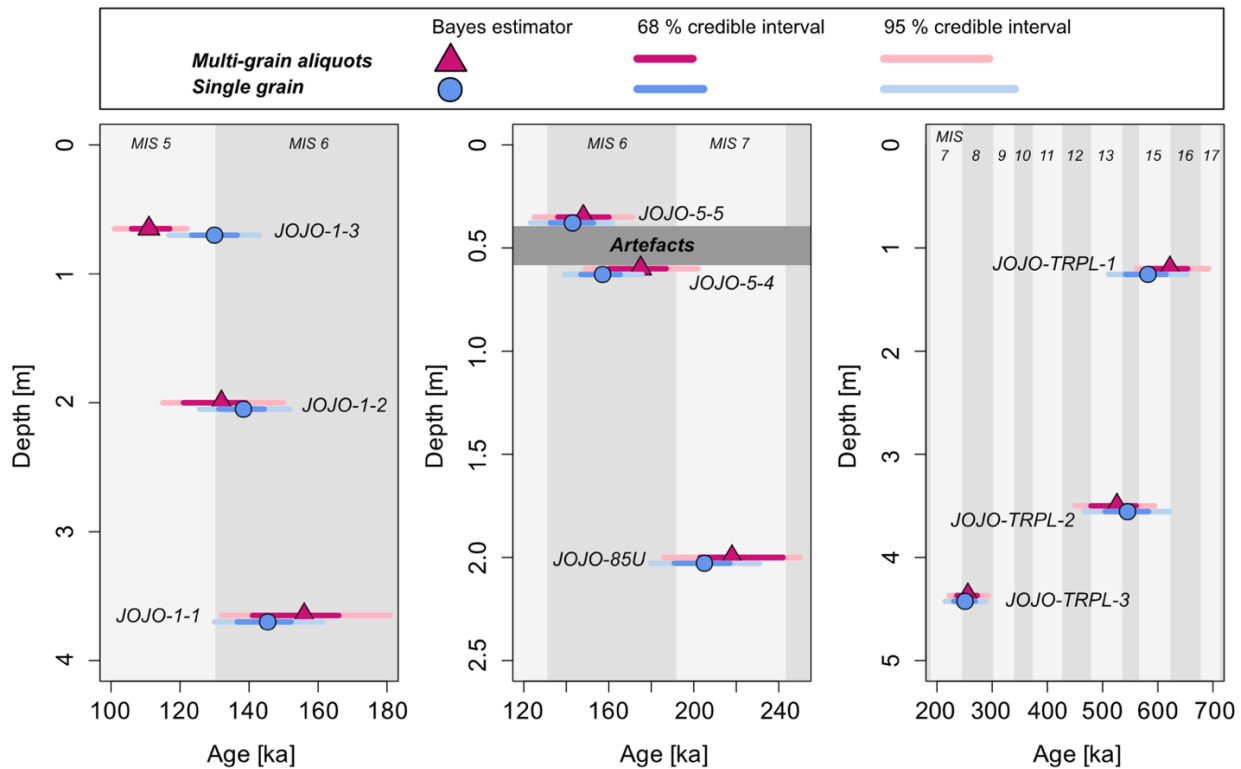
Fig. 56: Age depth plot of the three sediment profiles measured (profiles Jojosi-1, Jojosi-5, and Jojosi Triple Junction, from left to right). The ages displayed here were obtained using BayLum with stratigraphic constraints. Note: JOJO-TRPL is a cut-and-fill profile, meaning that the depth is not meaningful in terms of stratigraphic order, cf. Fig. 1. The shaded areas indicate marine isotope stages (MIS).
