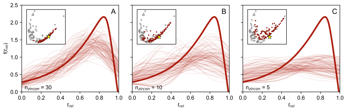
Figure 7. Bootstrap Kernel density plots showing results of bootstrap sampling of the theoretical zircon crystallisation distribution in a monotonically cooling magma reservoir derived from thermodynamic models (Keller et al., 2018) as shown by the thick red curve. The number of zircons sampled ( n_{zircon} ) ranges from 30 (left A) 30, 10 (centre B) 10, to 5 (right C) 5 and the thin translucent red curves show 100 iterations of sampling iterations. An uncertainty is added to each age as appropriate for a sample at 10 Ma. Inset plots show the PCA of the W_2 dissimilarity matrix of natural zircon U-Pb distributions (grey symbols) and where the 100 synthetic age distributions plot (red symbols) relative to the sampled distribution (star) .
