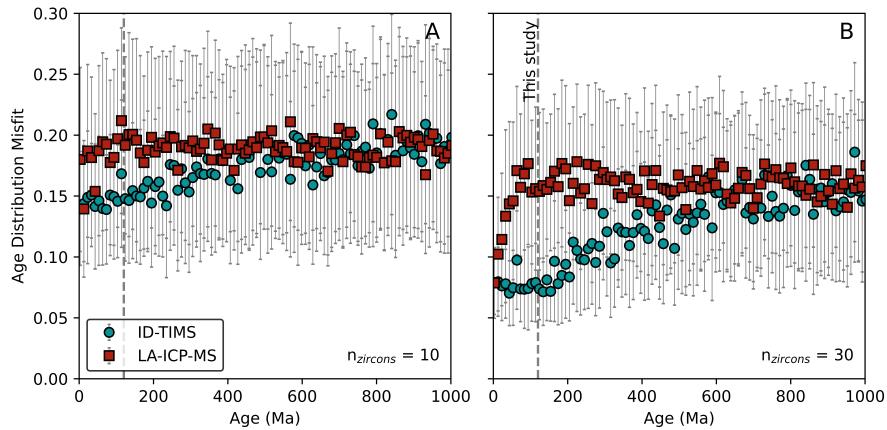
Figure 11. Comparison of the ability of ID-TIMS and LA-ICP-MS to capture the underlying zircon age distribution. At a given age, bootstrap forward modelling is applied on the monotonic cooling age distribution (Keller et al., 2018) and the Wasserstein distance is calculated between the sampled age distribution and the underlying distribution. At each age this is repeated 25 times and the mean W_2 is shown with the error bars showing the standard deviation. Vertical dashed line shows the maximum age of ID-TIMS distributions permitted in this study. This method is repeated for A) n_{zircon} = 10 and B) n_{zircon} = 30 .
