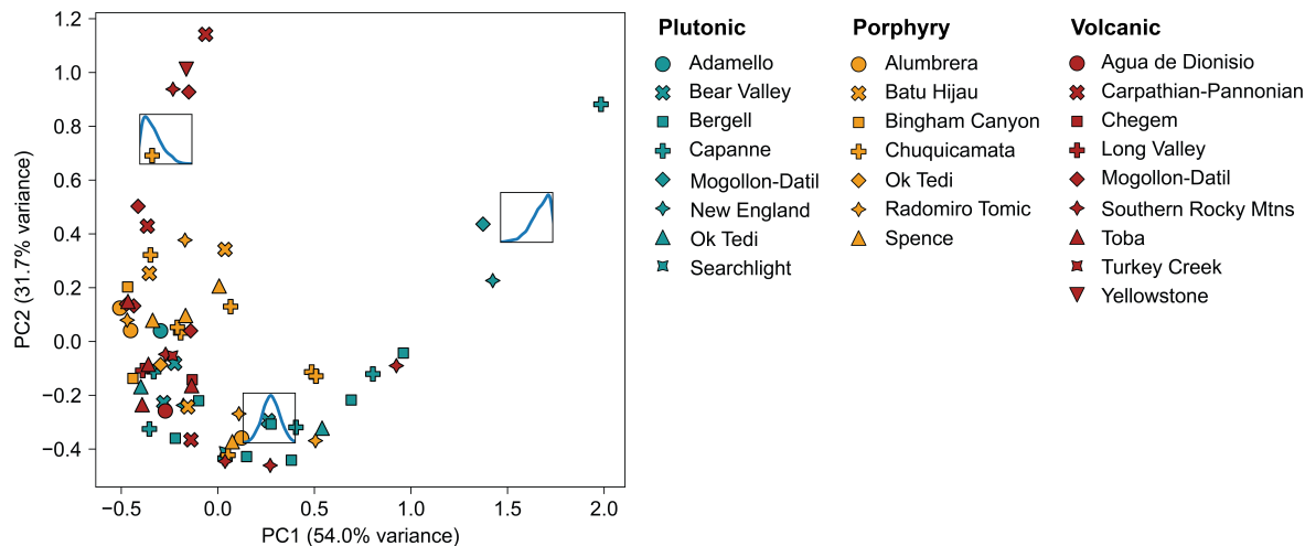
Figure 5. Results of PCA on the W_2 ID-TIMS zircon U-Pb dissimilarity matrix. Each data point indicates one U-Pb age distribution ( i.e. one sample or unit ) for a magmatic system. The percentage variance that each principal component accounts for is given. Three inset graphs represent KDEs of skew normal distribution with varying values of skew (-100, 0 and 100) for comparison with natural distributions.
