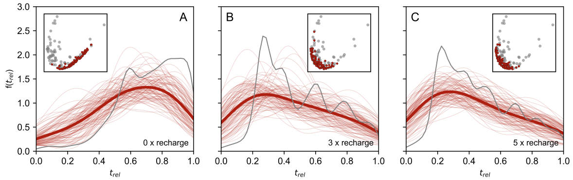
Figure 9. The Modelled kernel density curves showing the effect of repeated magma recharge on zircon age distributions. Underlying zircon age distributions produced with varying numbers of recharges of felsic melt into a felsic magma reservoir undergoing cooling and crystallisation. Underlying zircon age distributions (grey curves) are taken from Tavazzani et al. (2023b) for (A) 0, (B) 3, and (C) 5 recharge events during magma cooling. Thirty zircons are sampled from each on of the 100 sampled distributions and uncertainties are added as appropriate for 10 Ma old zircons (red curves). The average curve (thick opaque red) shows the average of the 100 synthetic age distributions and the progressive shift from old to young skew with increasing number of recharges. Insets show the location of these distributions (red symbols) in the PCA plot of the W_2 dissimilarity matrix of natural zircon U-Pb distributions (grey symbols).
