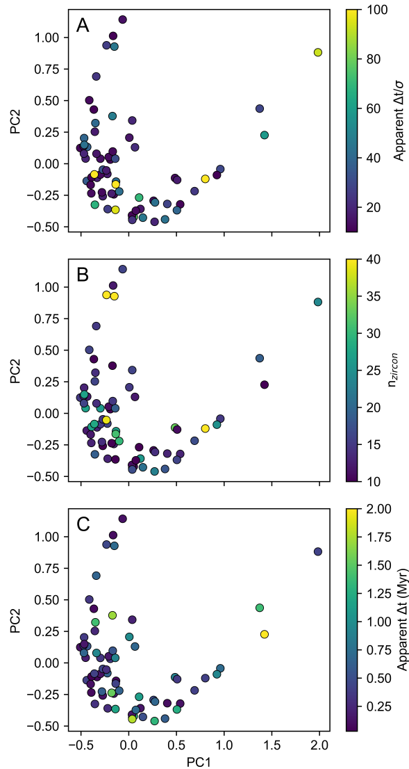
Figure 6. Plot of the PCA on the W_2 ID-TIMS zircon U-Pb dissimilarity matrix coloured by: (A) the ratio of zircon crystallisation duration and the mean analytical uncertainty (apparent \Delta t/\sigma ), (B) the number of zircons in the age spectrum ( n_{zircon} ) and (C) the duration of zircon crystallisation in Myr (apparent \Delta t ).
