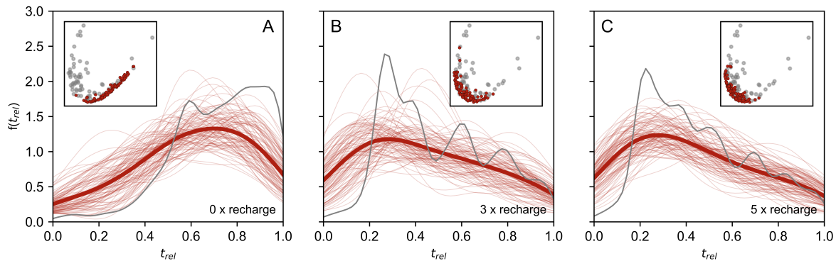
Figure 9. Modelled kernel density curves showing the effect of repeated magma recharge on zircon age distributions. Underlying zircon age distributions produced with varying numbers of recharges of felsic melt into a felsic magma reservoir undergoing cooling and crystallisation. Underlying zircon age distributions (grey curves) are taken from Tavazzani et al. (2023b) for (A) 0, (B) 3, and (C) 5 recharge events during magma cooling. Thirty zircons are sampled from each on of the 100 sampled distributions and uncertainties are added as appropriate for 10 Ma old zircons (red curves). The average curve (thick opaque red) shows the average of the 100 synthetic age distributions and the progressive shift from old to young skew with increasing number of recharges. Insets show the location of these distributions (red symbols) in the PCA plot of the W_2 dissimilarity matrix of natural zircon U-Pb distributions (grey symbols).
