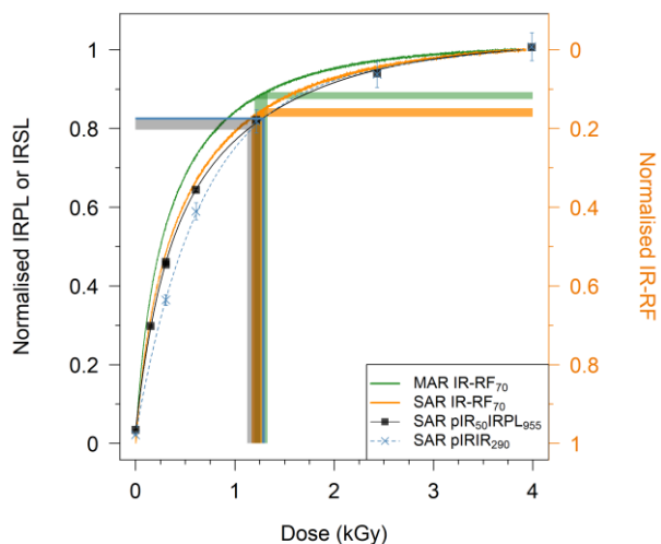
765 Figure 9: DRC shape comparison of representative aliquots of Gi326. The pIR_{50}IRPL_{955} and the pIR_{90}IR_{290} curves are double exponential functions fitted to the sensitivity corrected signals ( L_x/T_x ) of 7–8 regenerative doses each, including a repeated dose point (~300 Gy). All curves were normalised to their maximum values. Before normalisation, a background was subtracted from the IR-RF curves, corresponding to the median value of the last 100 channels (~60 Gy). The IR-RF curves decrease with dose, so they were plotted on an inverted axis (right-hand side) to allow for a direct comparison. The shaded 770 regions indicate the 1\sigma range around the four mean D_e values and their projection onto the corresponding DRC.
