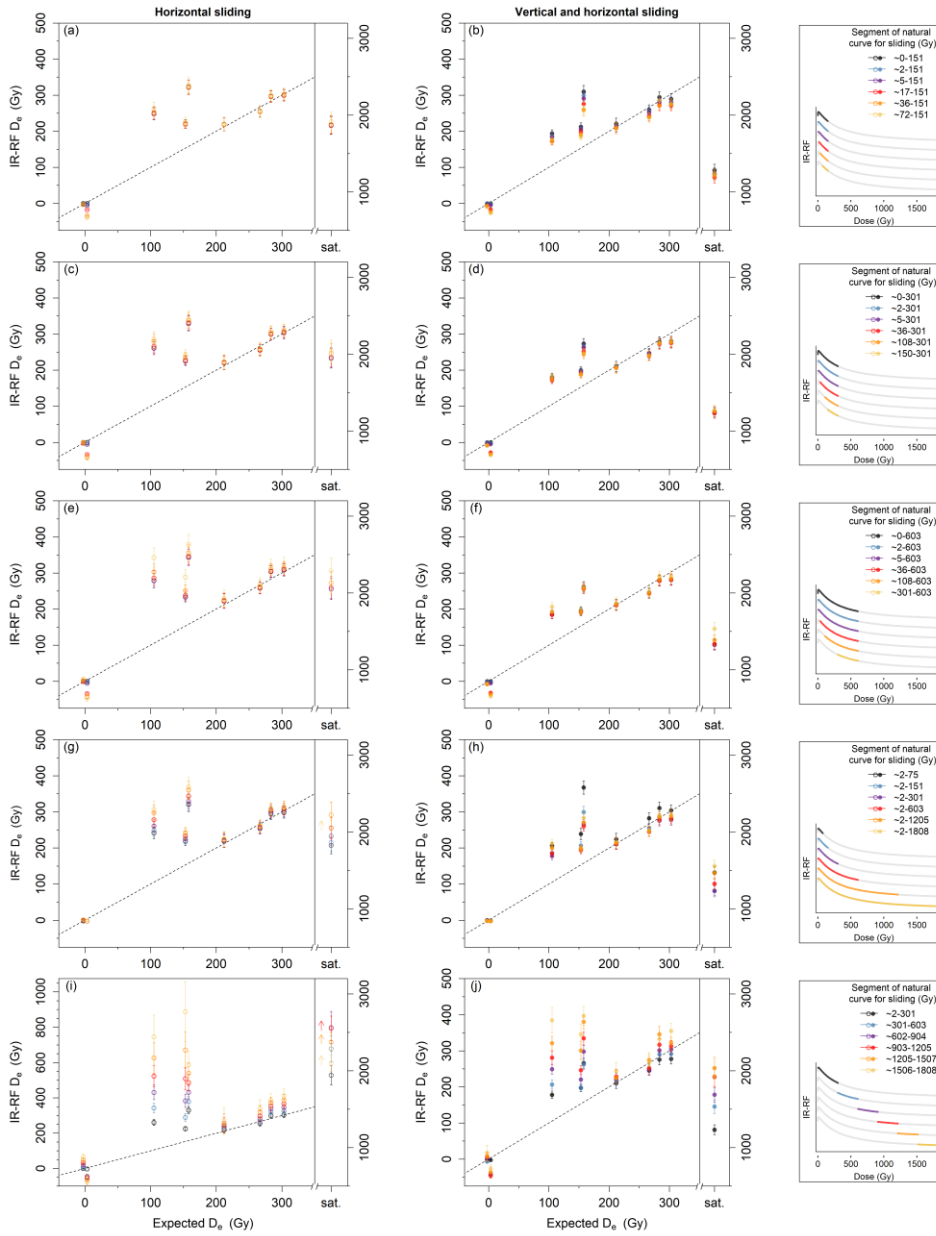
Figure 5: Comparison of IR-RF 70 mean D_e values using fixed segments of the natural dose curve and (a, c, e, g, i) only horizontal sliding or (b, d, f, h, j) vertical and horizontal sliding. For clarity, the used segments of a representative natural dose curve (sample 092202) are shown in the legend box to the right of the corresponding plots. Note that a 5 Gy interval was placed between the expected doses of the two modern samples to aid visualization. The D_e for the field-saturated sample Gi326 is shown on the right-hand y-axis in each plot; its expected D_e is 'saturated' (sat.). The dashed line indicates the 1:1 line. (e, g) Arrows indicate a minimum estimate caused by the limit of the regenerative dose curve.
