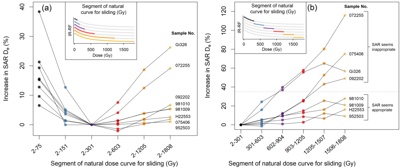
775 Figure 10: Test of progressive sensitivity changes during the IR-RF 70 natural dose curve measurement. D_e values of non- 780 modern samples were obtained using fixed segments of the natural dose curve according to the x-axis labels with vertical and horizontal sliding (same data and colours as in (a) Fig. 5h and (b) Fig. 5j). The increase in D_e is relative to that obtained from the segment 2–301 Gy. (b) The dashed line (35% increase) separates samples that produce D_e values within 2\sigma of the expected dose and those that do not.
