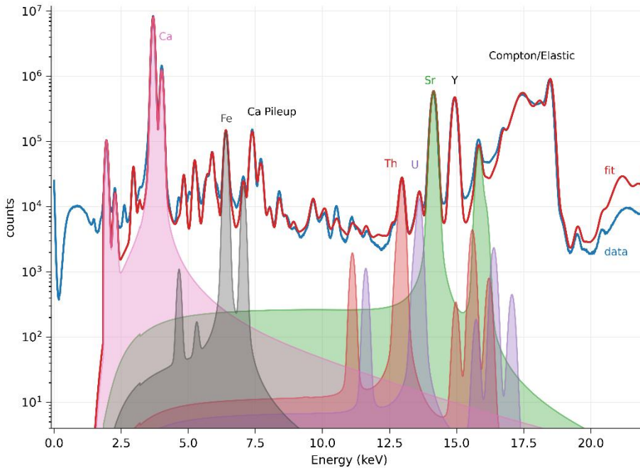
Figure A1. Measured XRF spectrum for all detectors and pixels from one slice of MGB5-2, before correcting for self-absorption. Fitted eigenfunctions for selected elements are shown.
