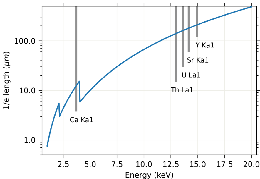
545 Figure B1. Energy (keV) vs 1/e length ( \mu\text{m} ). \mu(E) is from the Python library xraydb.
