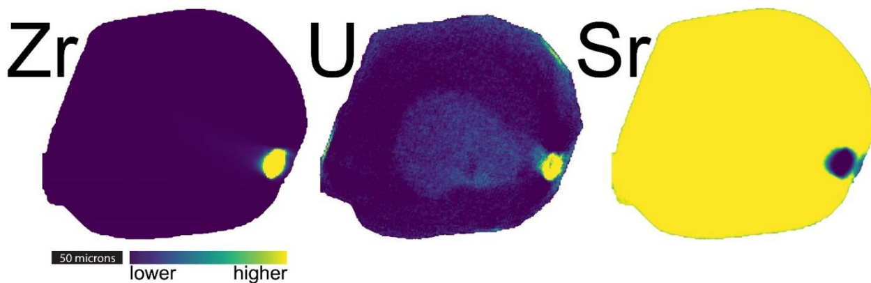
Figure 8. Three visualizations of a zircon inclusion in a single tomographic slice of an apatite crystal (AP1). The color scale is relative and designed to clearly distinguish between zircon inclusion and apatite crystal in Zr (left) and U (center), and Sr (right). This figure shows the same virtual slice as that in Figure 2F.
